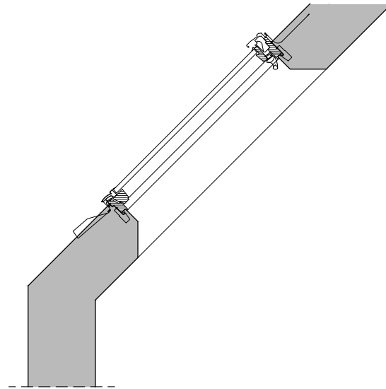
SECTIONAL DETAIL RECOMMENDED LINING
