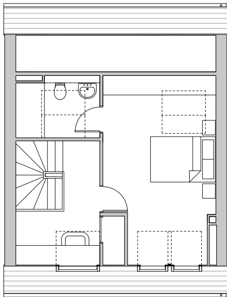
FLOOR PLAN AFTER
