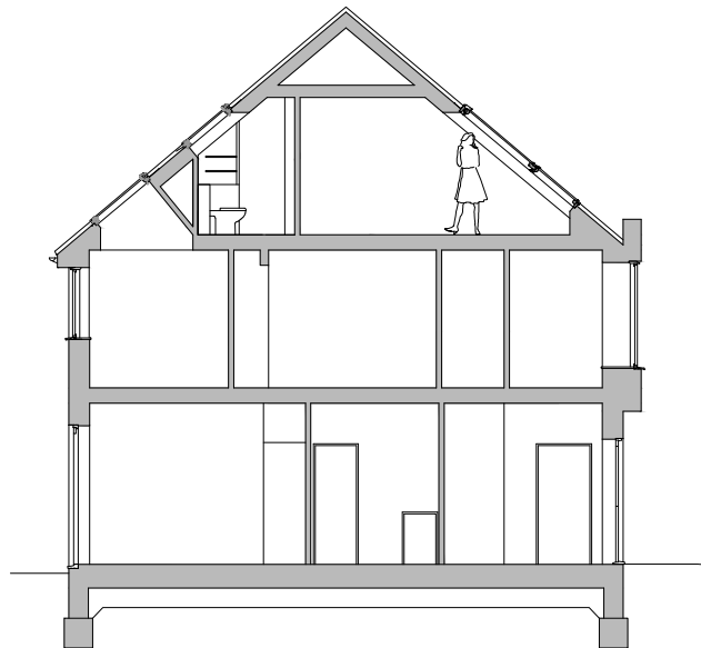
SECTION AFTER
