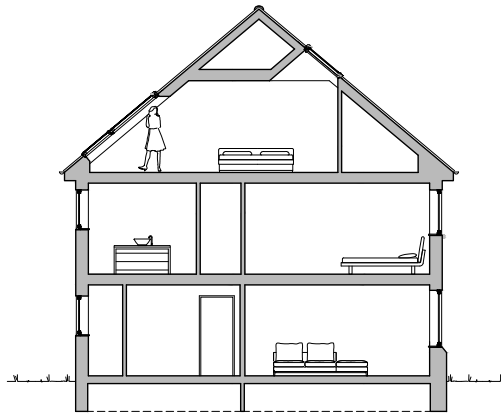
SECTION AFTER
