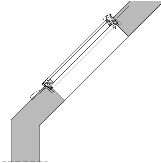
SECTIONAL DETAIL SUB-OPTIMAL LINING
