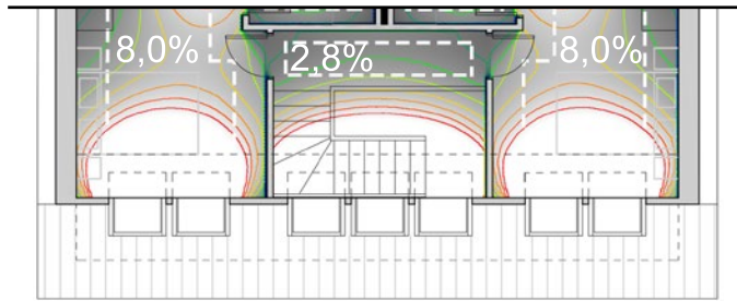
FLOOR PLAN & DAYLIGHT ANALYSIS AFTER
