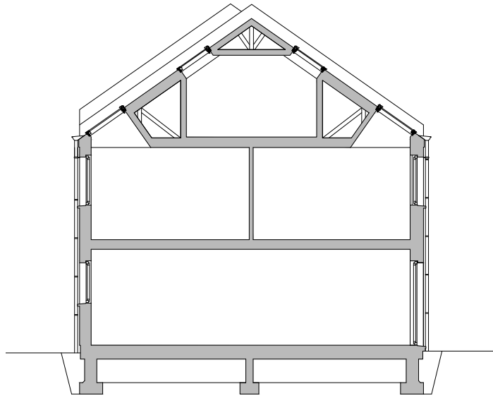
SECTION AFTER
