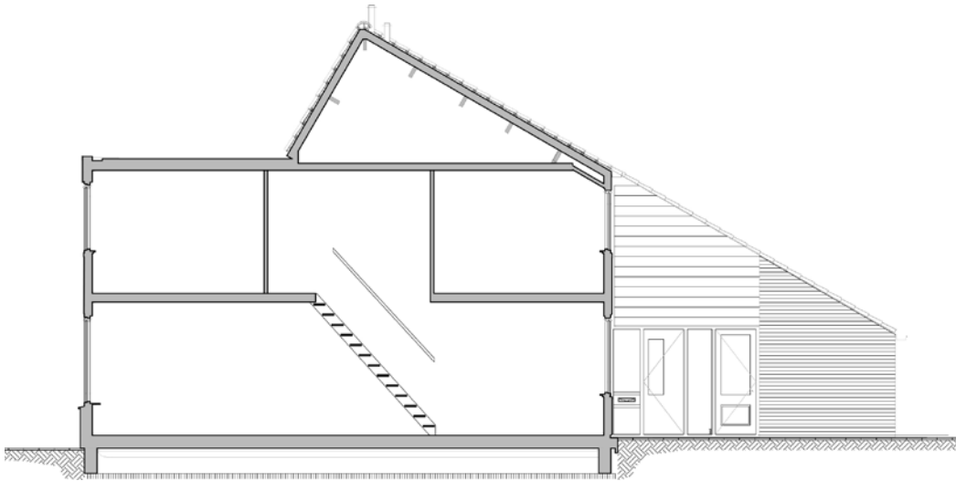
SECTION BEFORE
