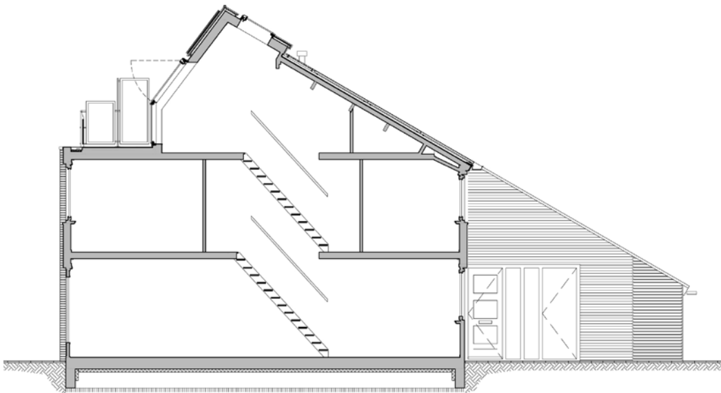
SECTION AFTER
