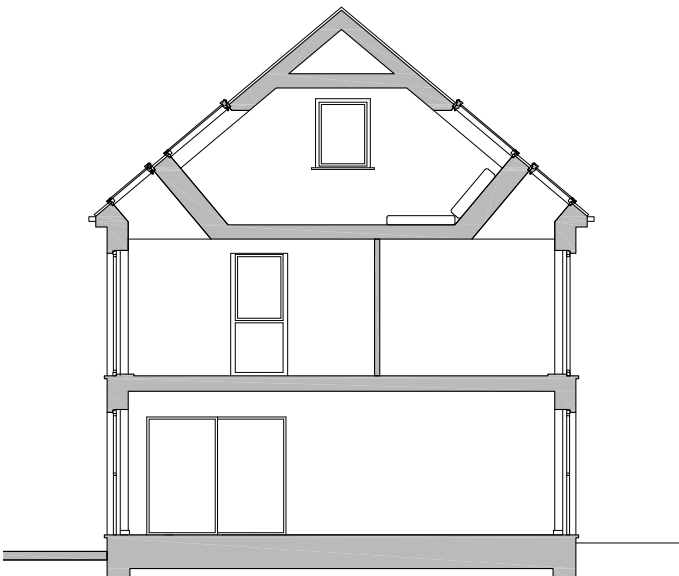
SECTION AFTER
