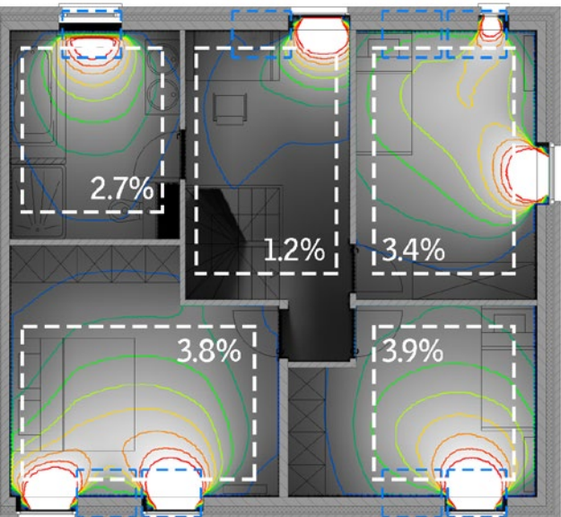
DAYLIGHT ANALYSIS AFTER
