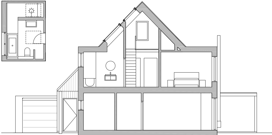
FLOOR PLAN AND SECTION
