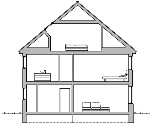
SECTION BEFORE
