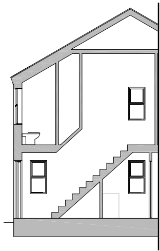
SECTION BEFORE
