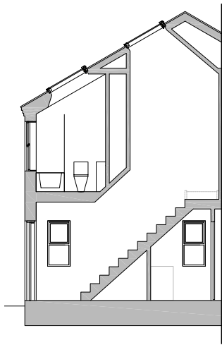
SECTION AFTER
