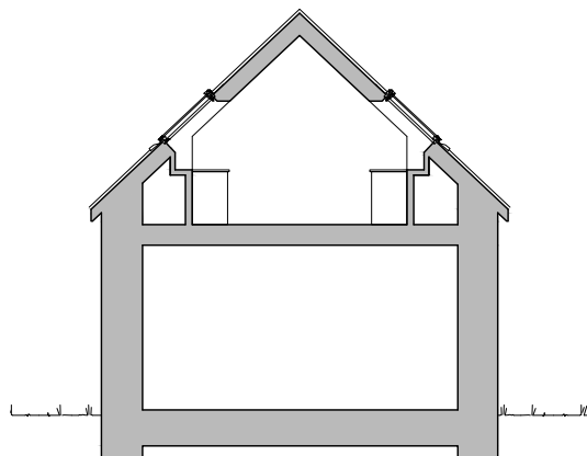
SECTION AFTER
