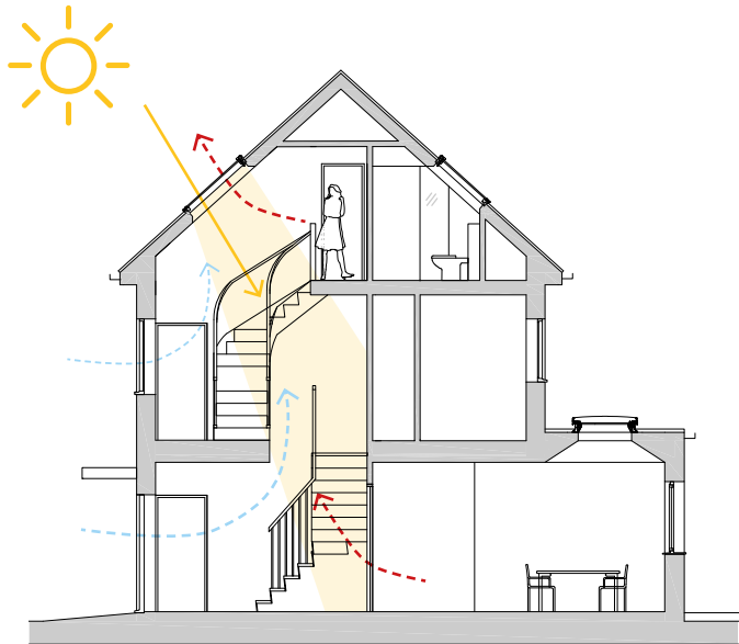
SECTION AFTER
