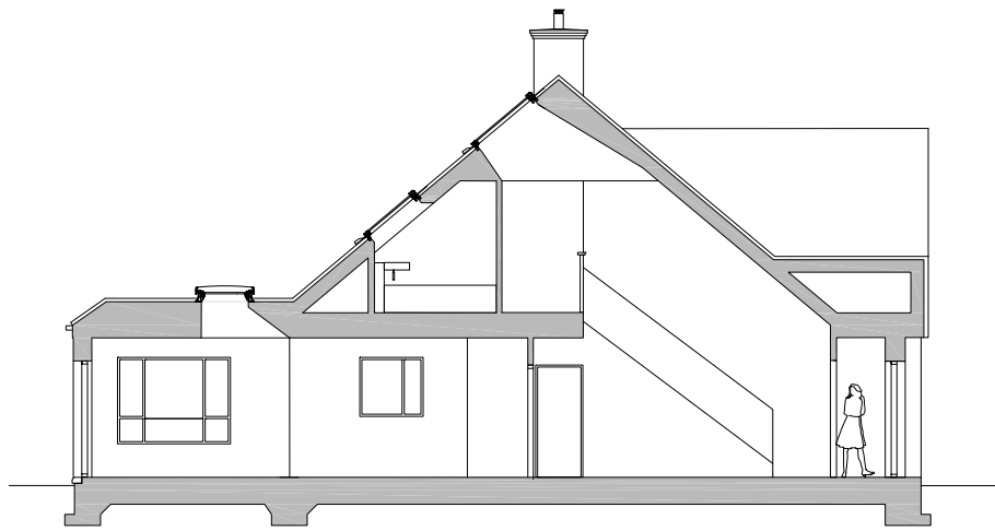
SECTION AFTER
