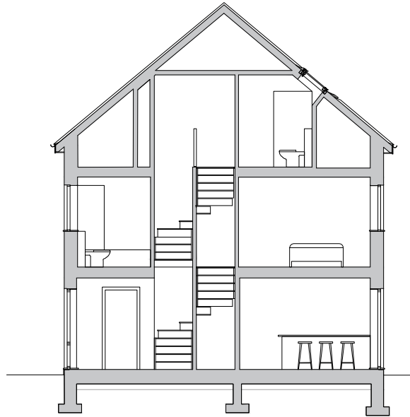
SECTION BEFORE
