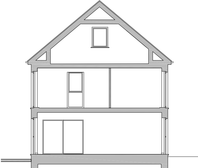
SECTION BEFORE
