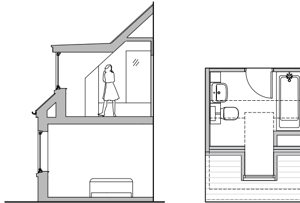
SECTION & PLAN BEFORE
