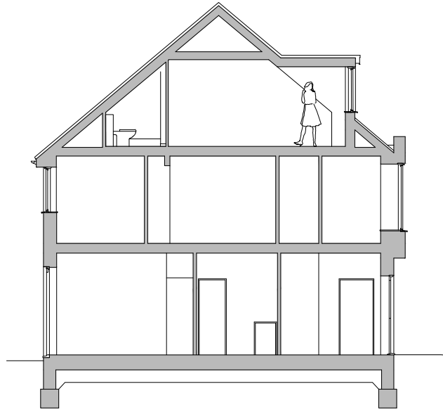
SECTION BEFORE
