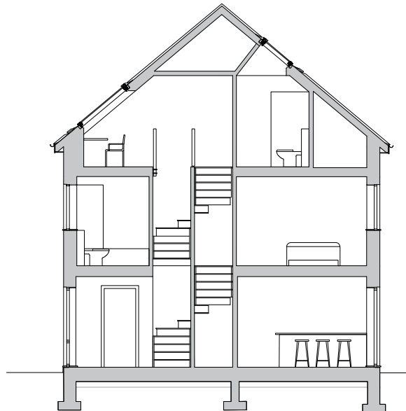
SECTION AFTER
