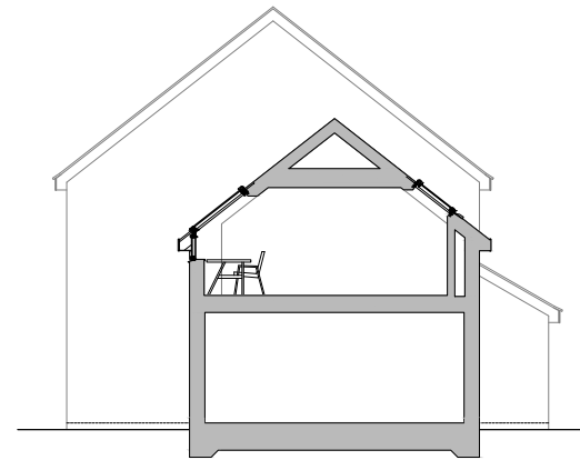
SECTION AFTER
