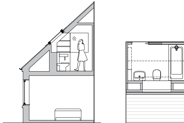
SECTION & PLAN AFTER
