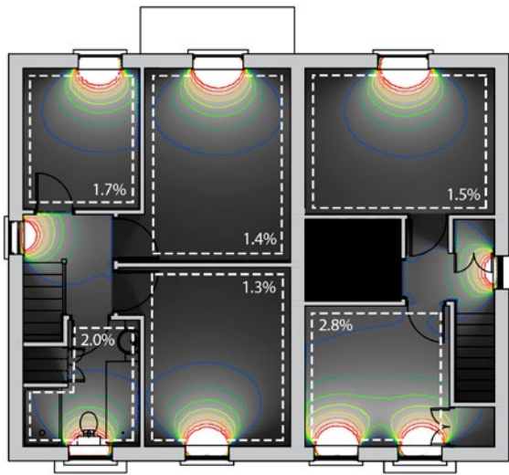
DAYLIGHT ANALYSIS BEFORE
